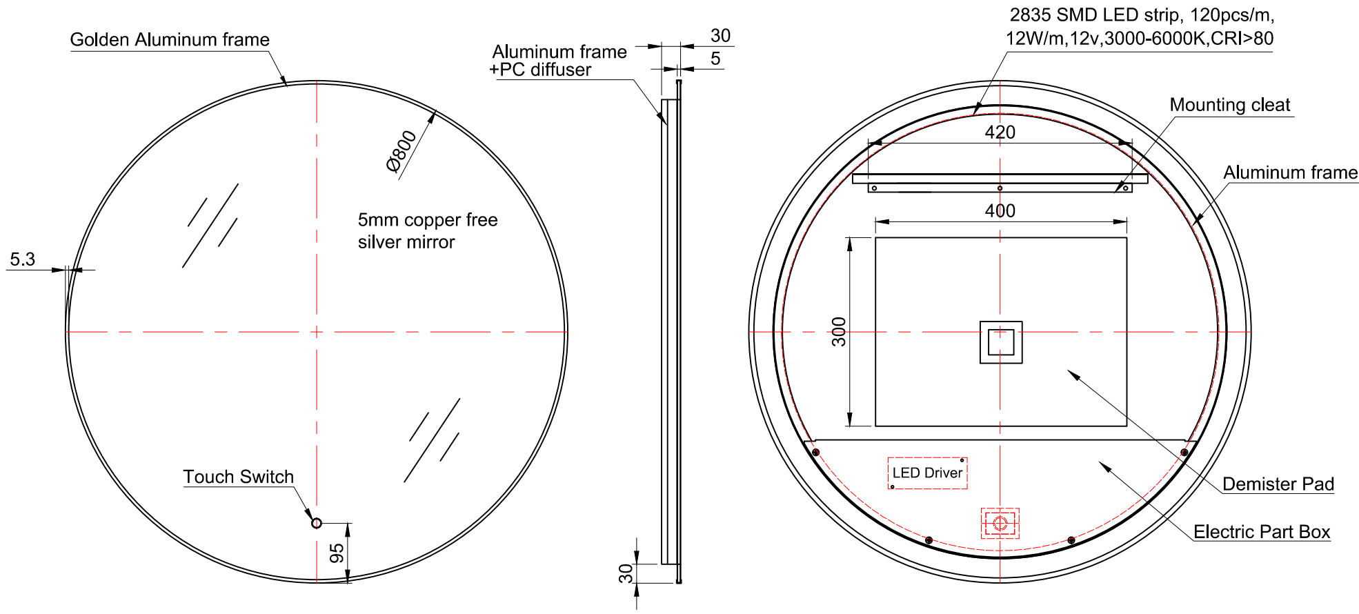
BACK VIEW
