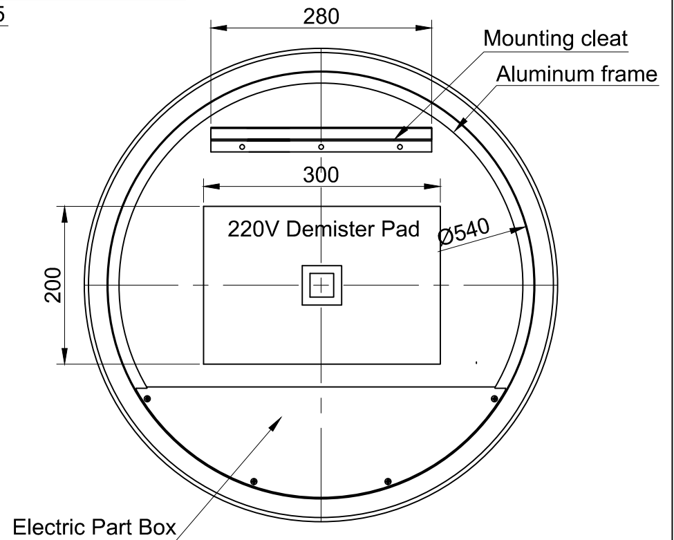
BACK VIEW
