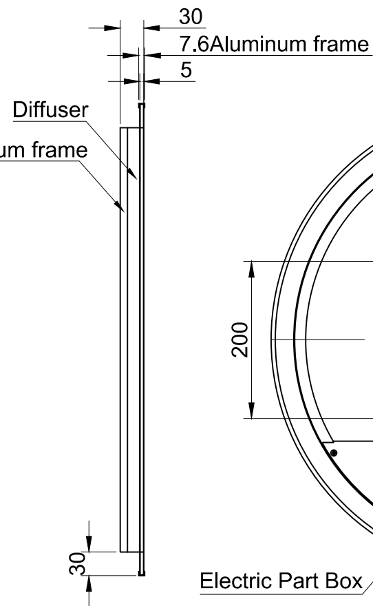
SIDE VIEW
