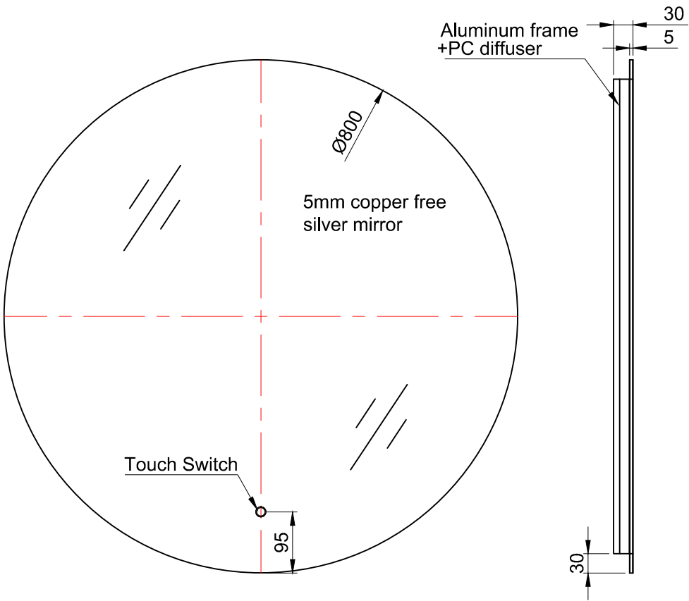
FRONT VIEW
