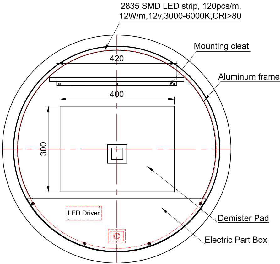
BACK VIEW
